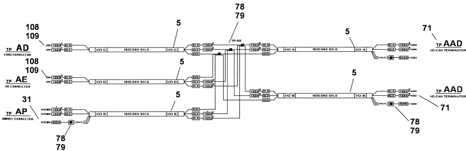
CABLE DETAIL I/O CAN A,B,C,D,E CONTROL MODULE PROPRIETARY CABLE
